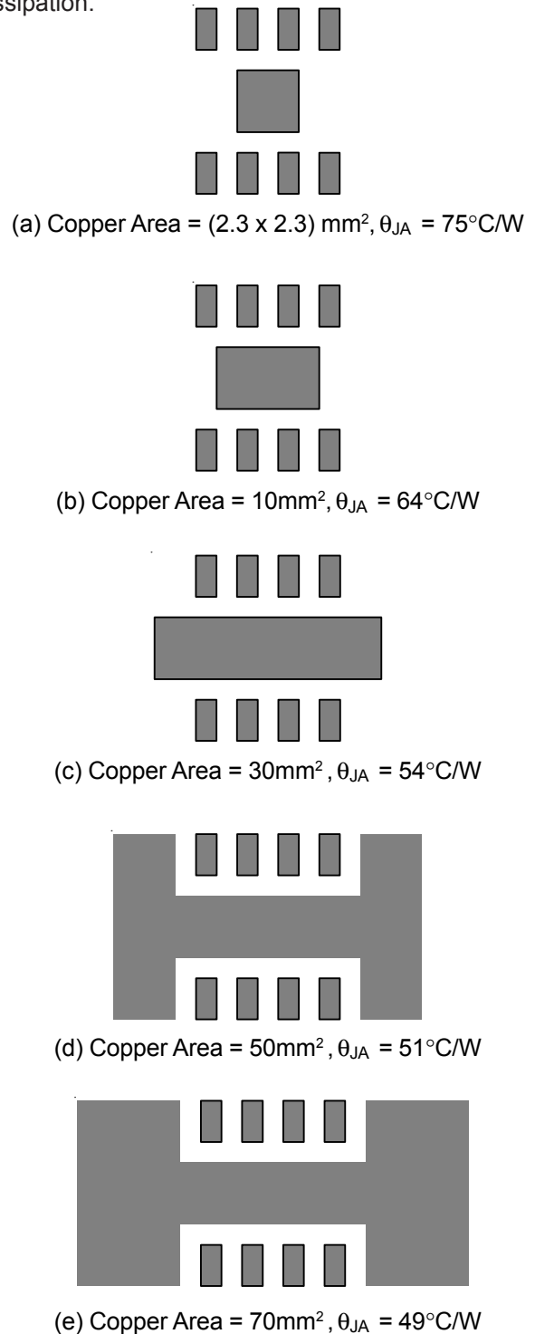
Figure 7. Thermal Resistance vs. Copper Area Layout Design
